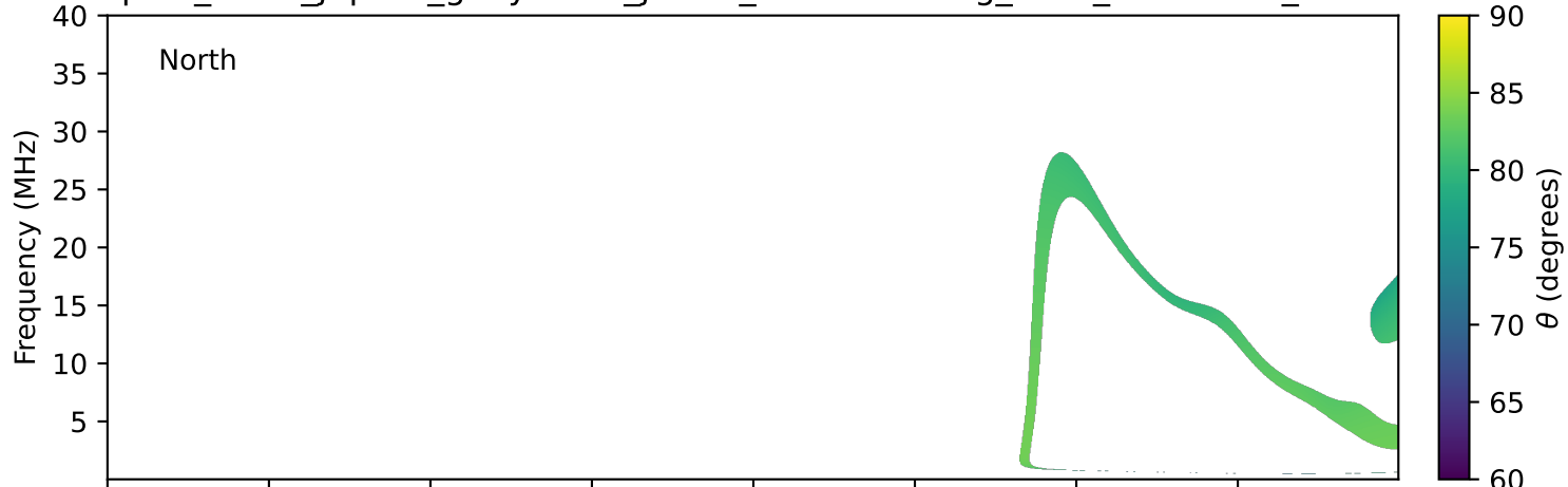
expres_earth_jupiter_ganymede_jrm33_lossc-wid1deg_3kev_20251123_v11.cdf
