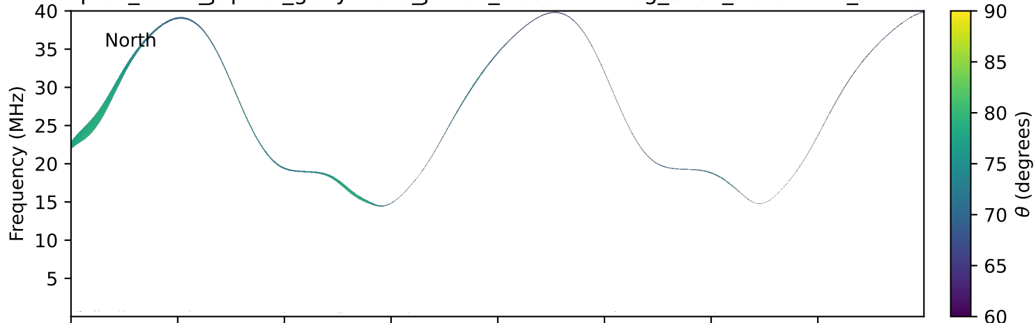
expres_earth_jupiter_ganymede_jrm33_lossc-wid1deg_3kev_20251117_v11.cdf
