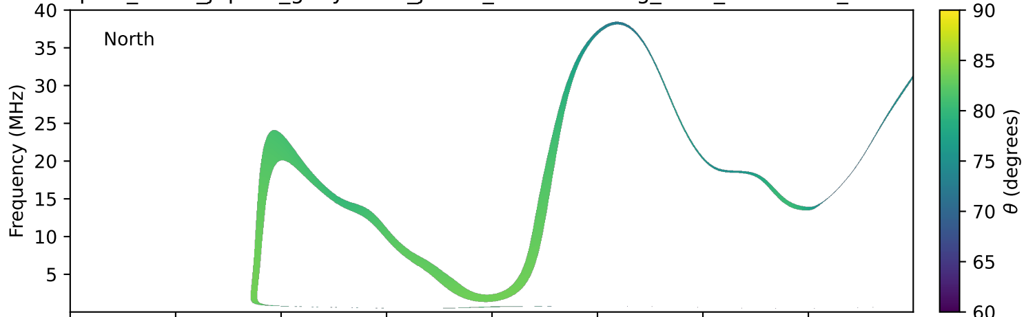
expres_earth_jupiter_ganymede_jrm33_lossc-wid1deg_3kev_20251102_v11.cdf
