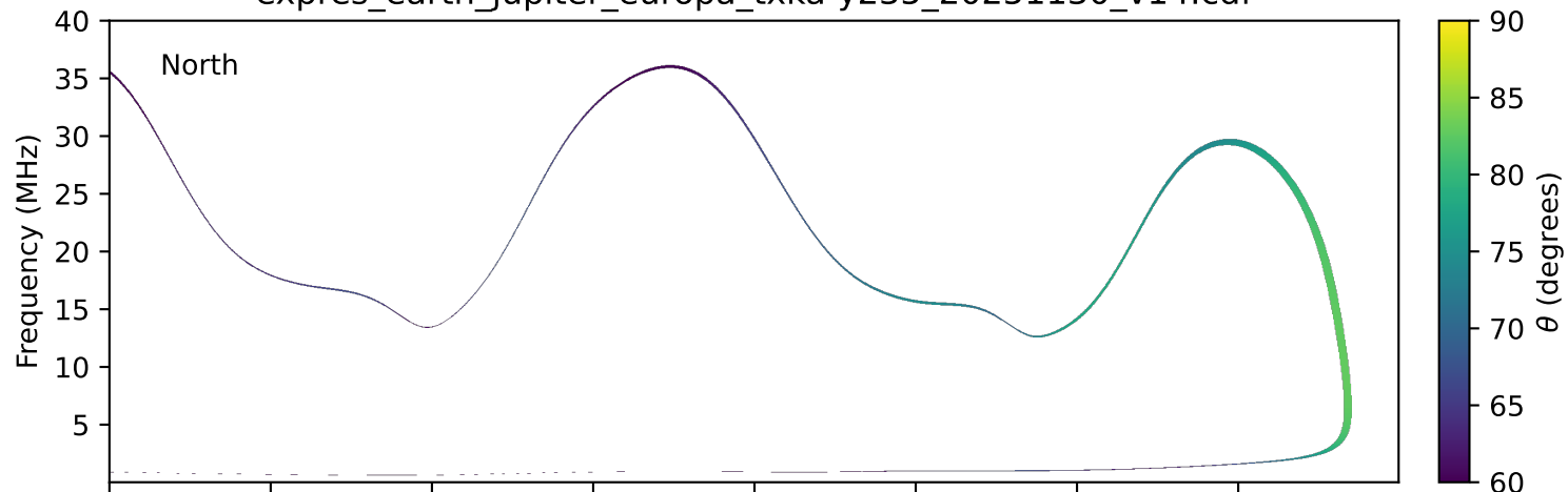
expres_earth_jupiter_europa_txka-y235_20251130_v14.cdf
