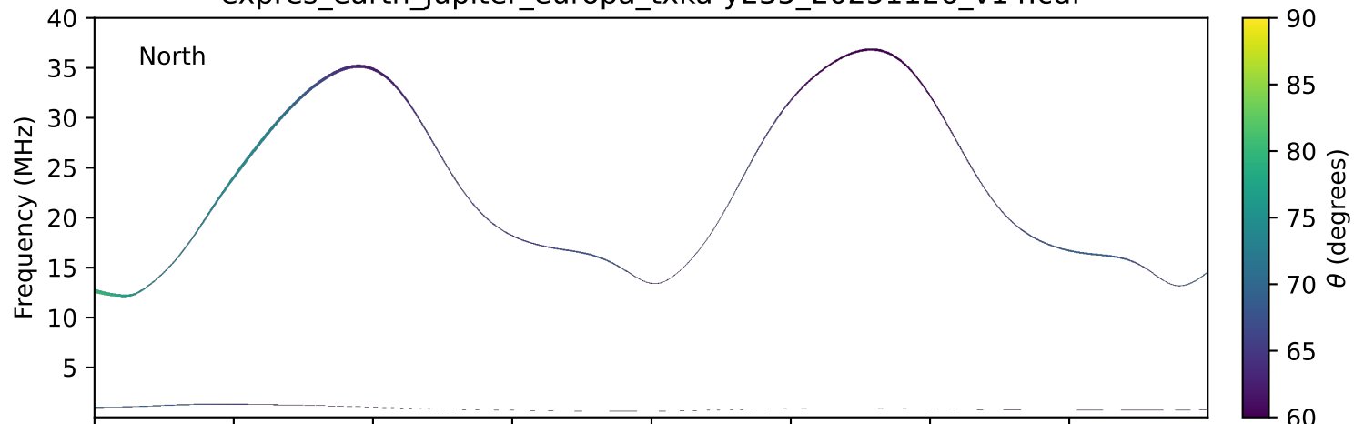
expres_earth_jupiter_europa_txka-y235_20251126_v14.cdf
