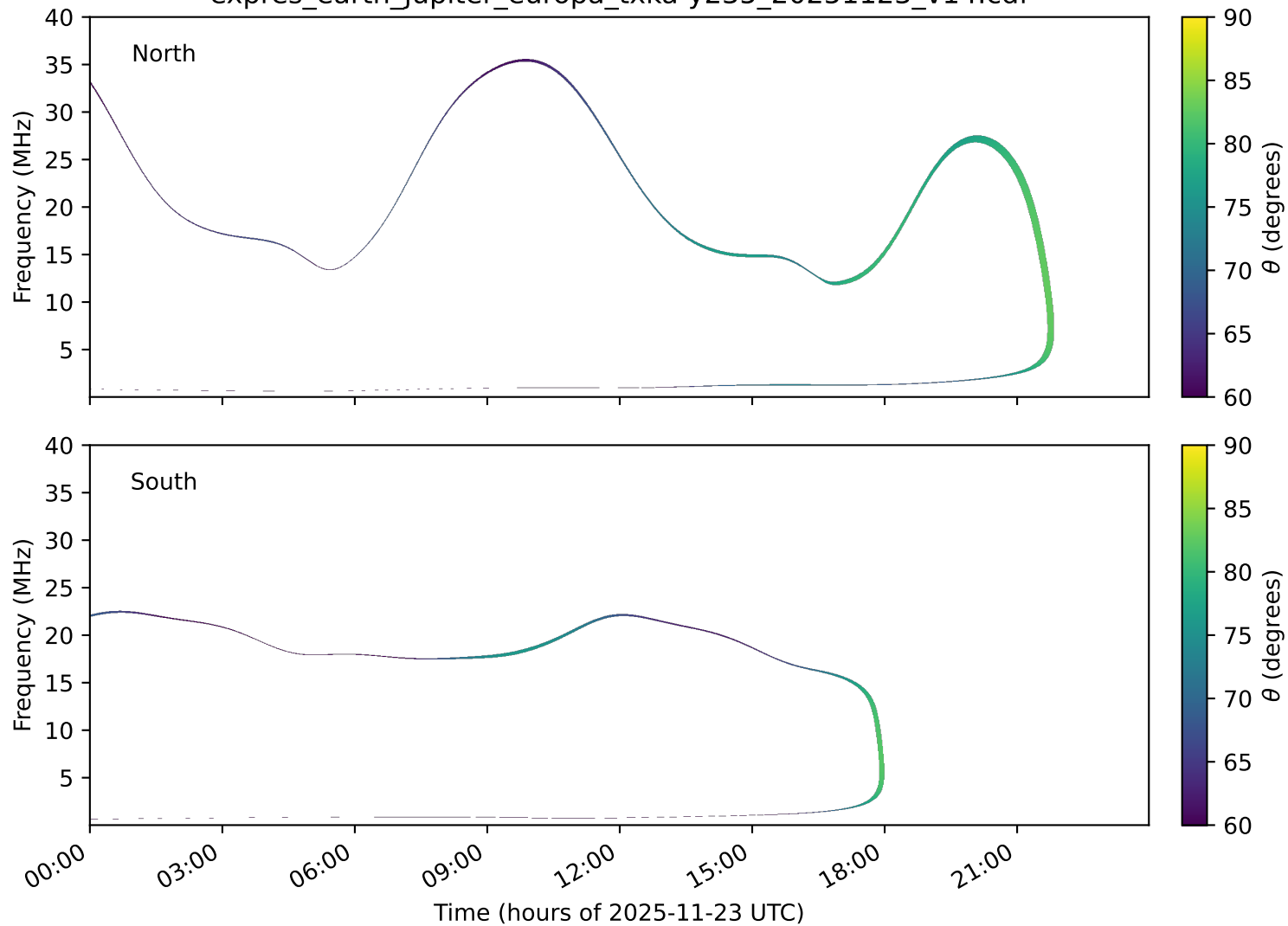
expres_earth_jupiter_europa_txka-y235_20251123_v14.cdf
