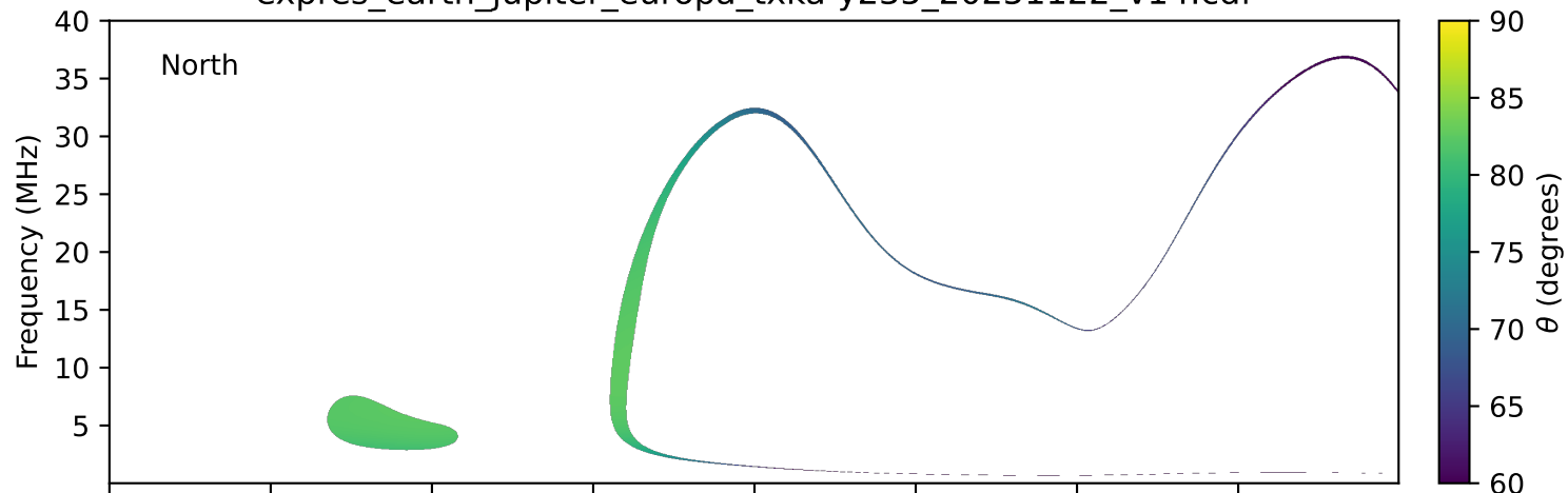
expres_earth_jupiter_europa_txka-y235_20251122_v14.cdf
