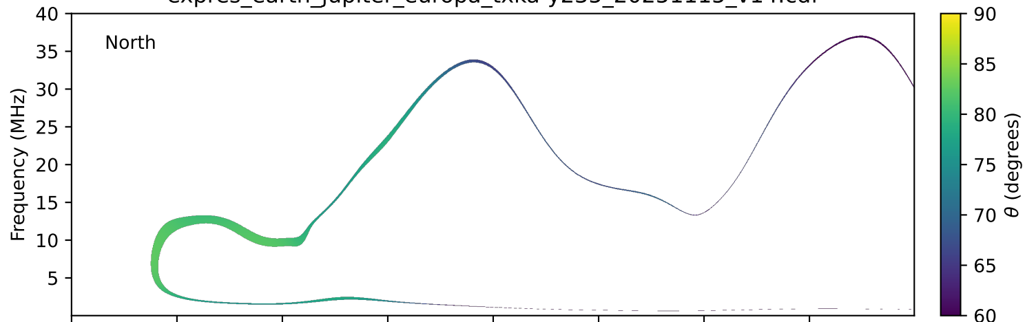
expres_earth_jupiter_europa_txka-y235_20251115_v14.cdf
