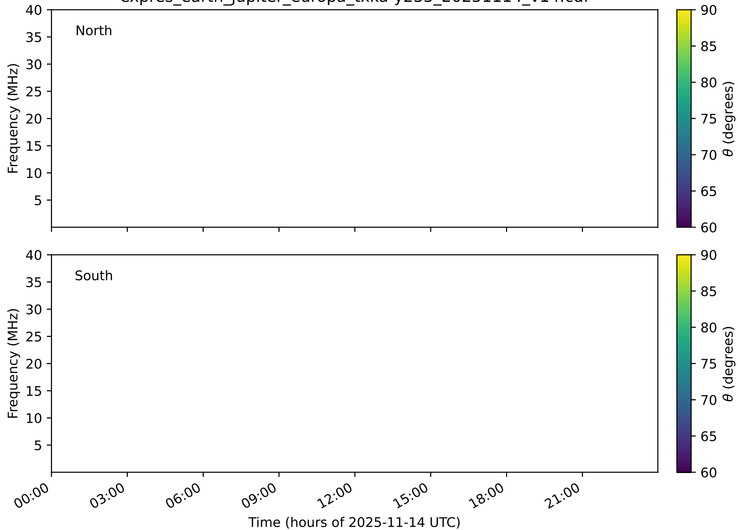
expres_earth_jupiter_europa_txka-y235_20251114_v14.cdf
