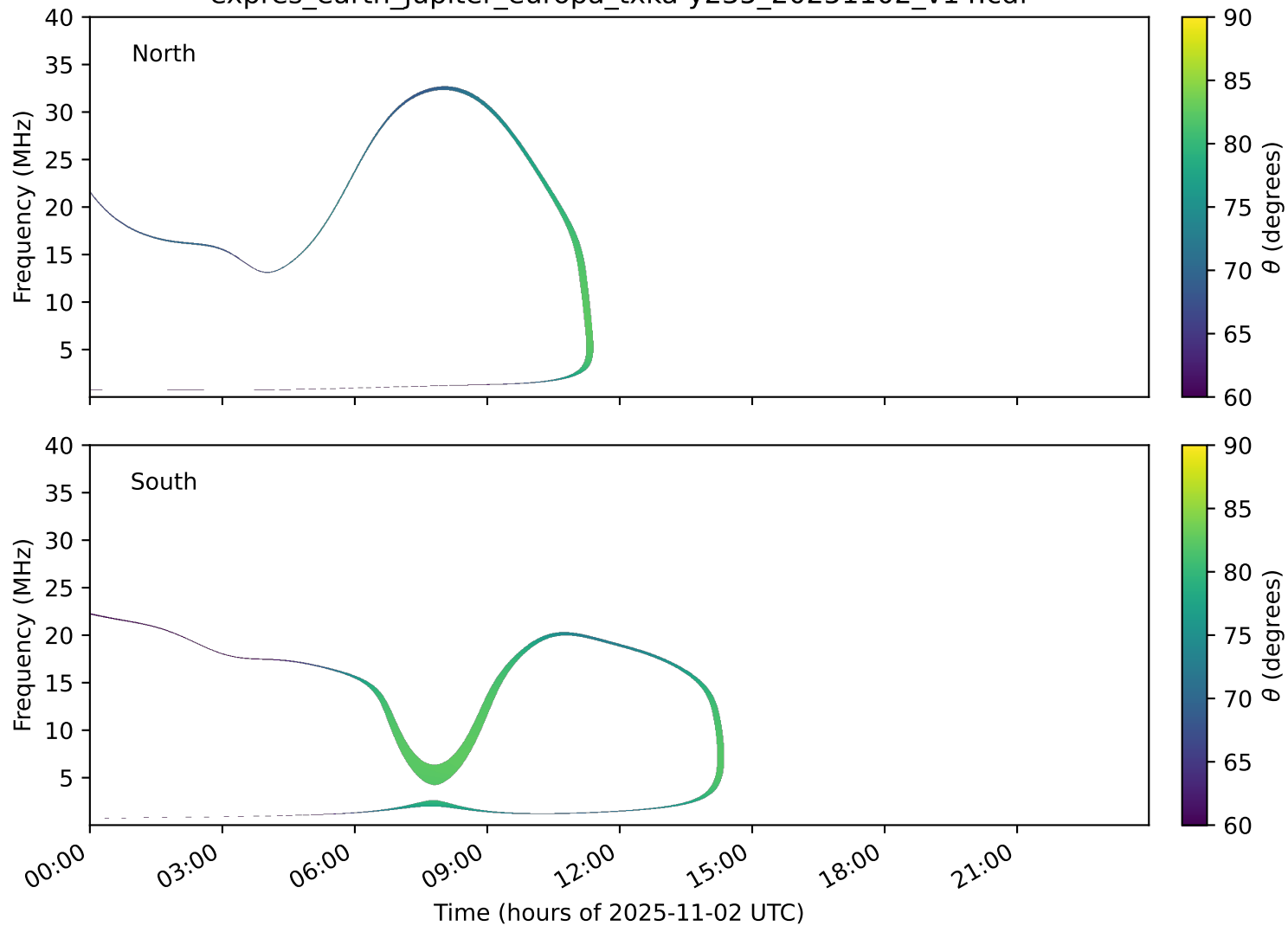
expres_earth_jupiter_europa_txka-y235_20251102_v14.cdf
