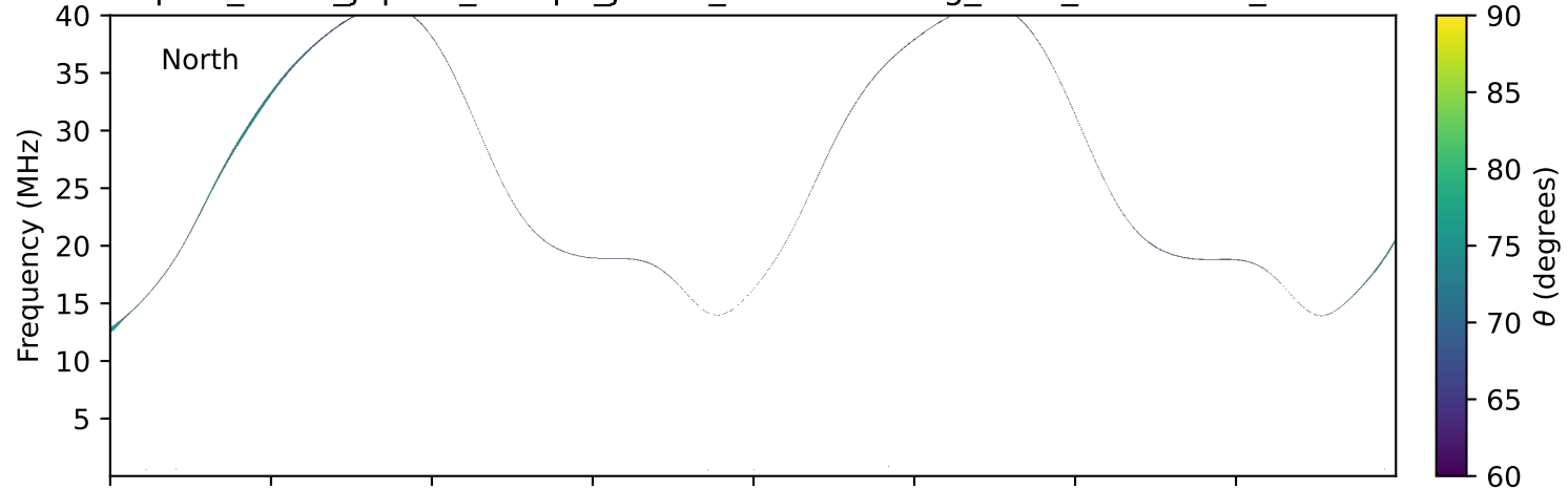
expres_earth_jupiter_europa_jrm33_lossc-wid1deg_3kev_20251119_v11.cdf
