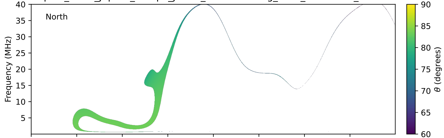
expres_earth_jupiter_europa_jrm33_lossc-wid1deg_3kev_20251115_v11.cdf
