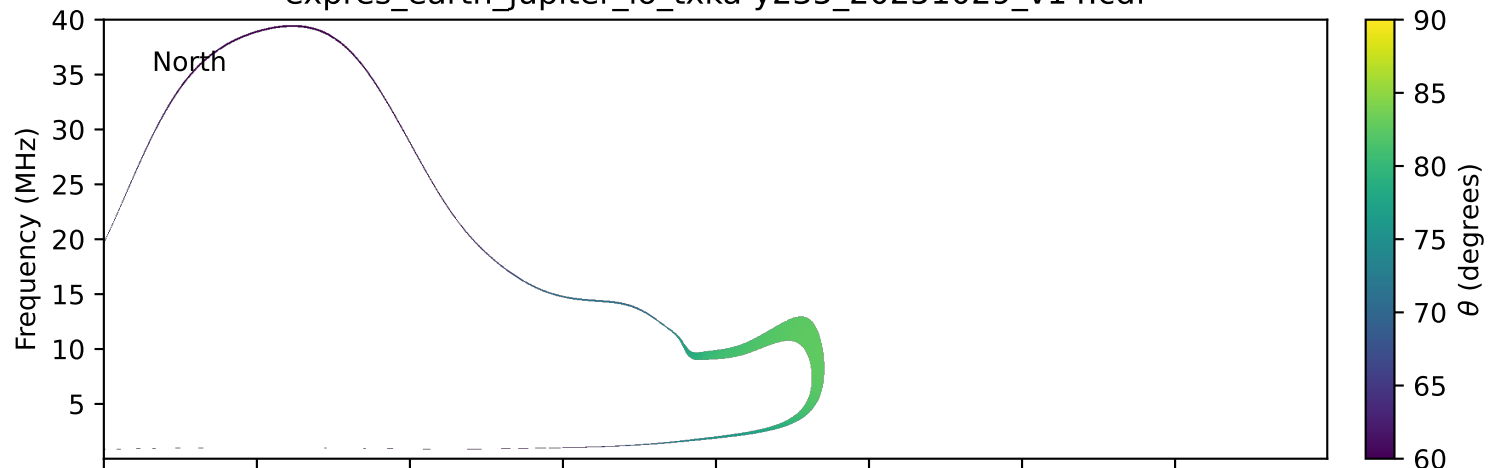
expres_earth_jupiter_io_txka-y235_20251029_v14.cdf
