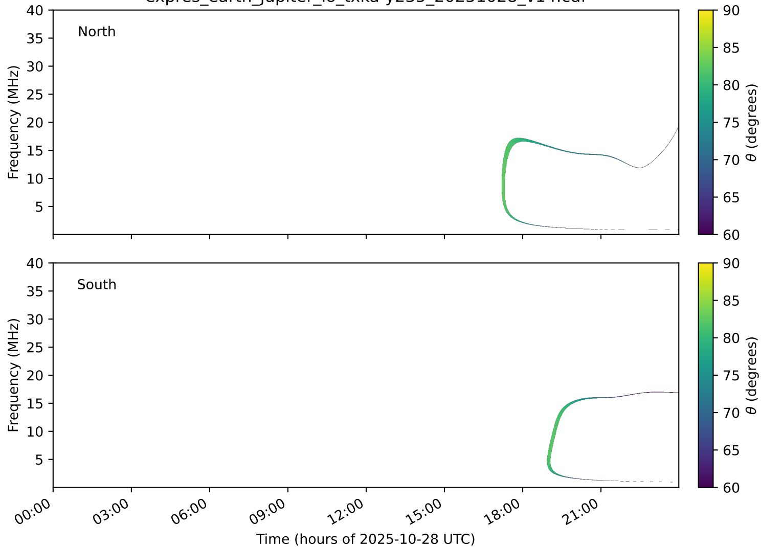
expres_earth_jupiter_io_txka-y235_20251028_v14.cdf
