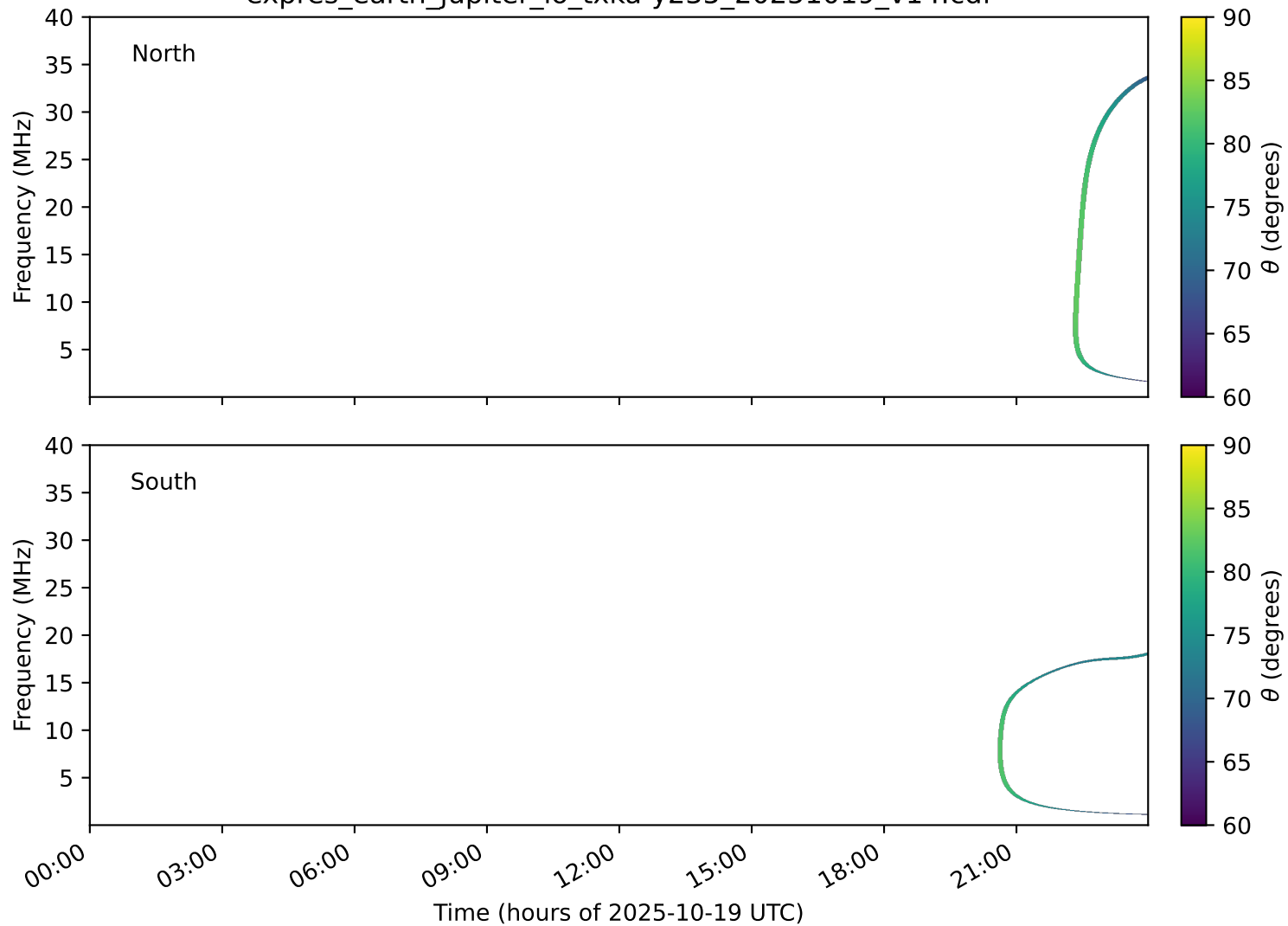
expres_earth_jupiter_io_txka-y235_20251019_v14.cdf
