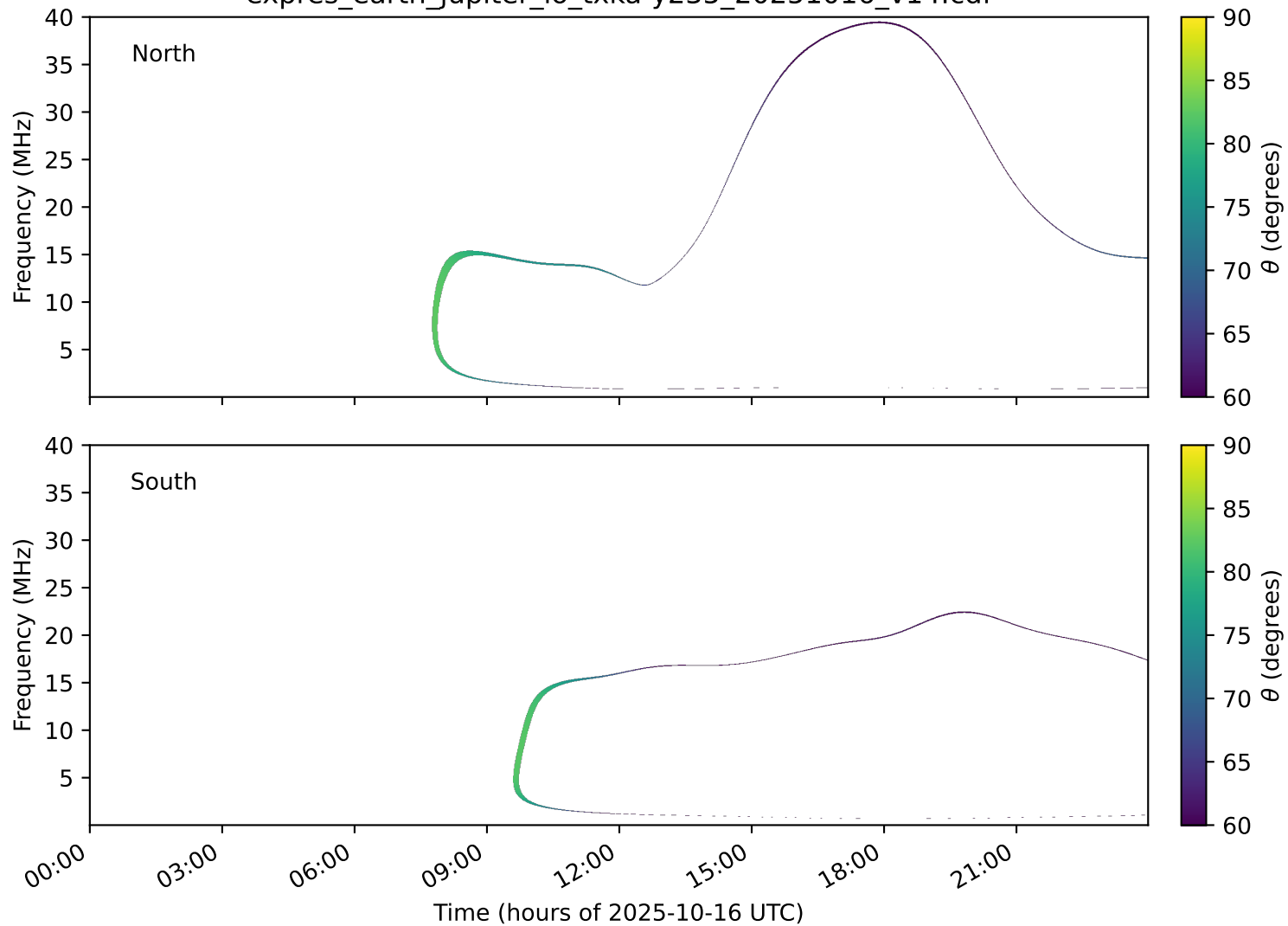
expres_earth_jupiter_io_txka-y235_20251016_v14.cdf
