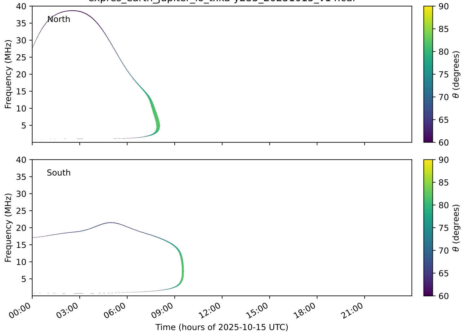
expres_earth_jupiter_io_txka-y235_20251015_v14.cdf
