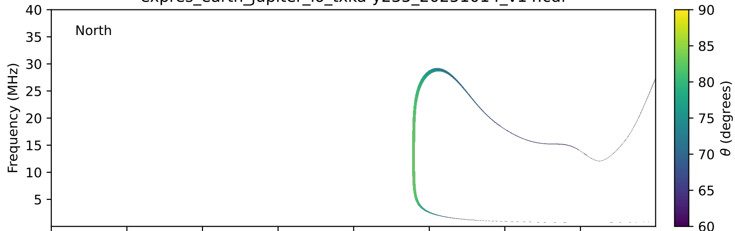
expres_earth_jupiter_io_txka-y235_20251014_v14.cdf
