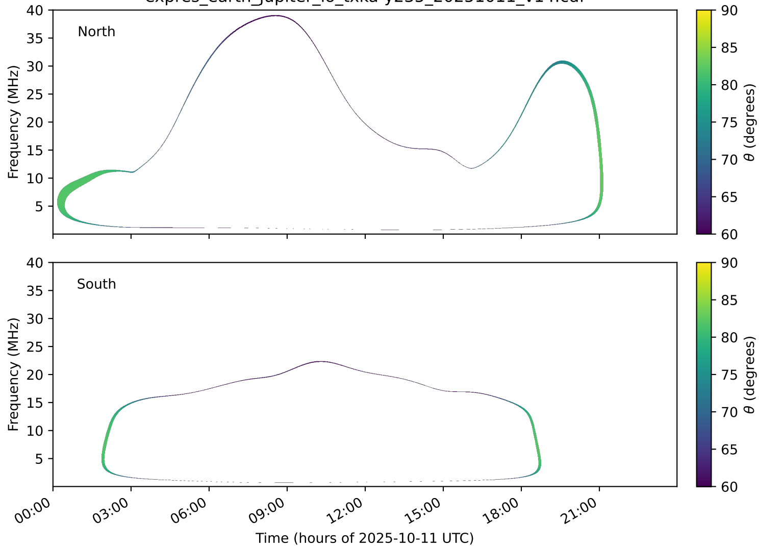
expres_earth_jupiter_io_txka-y235_20251011_v14.cdf
