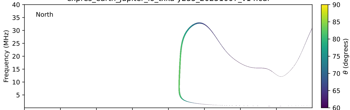
expres_earth_jupiter_io_txka-y235_20251007_v14.cdf
