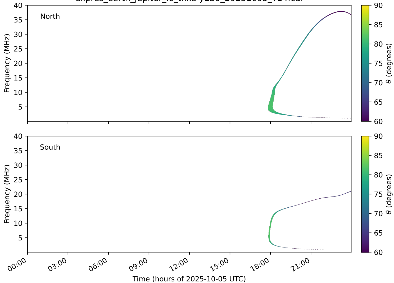
expres_earth_jupiter_io_txka-y235_20251005_v14.cdf
