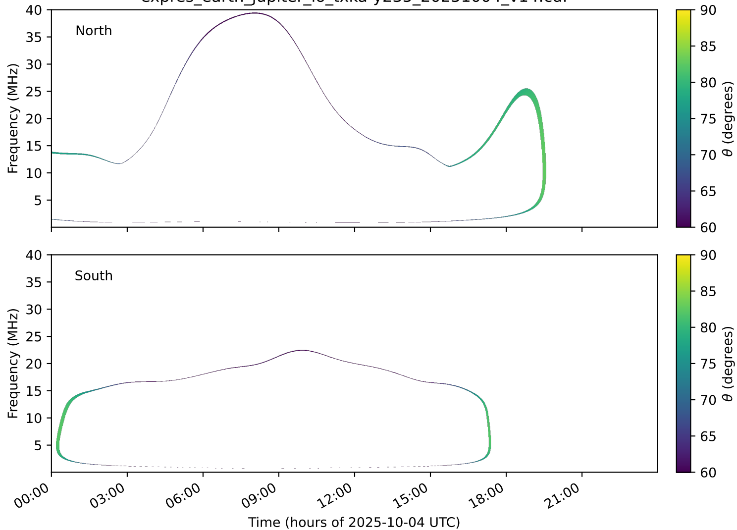
expres_earth_jupiter_io_txka-y235_20251004_v14.cdf
