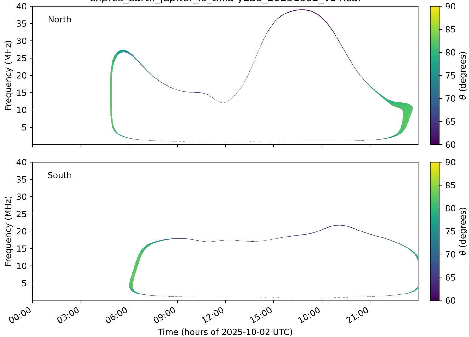
expres_earth_jupiter_io_txka-y235_20251002_v14.cdf
