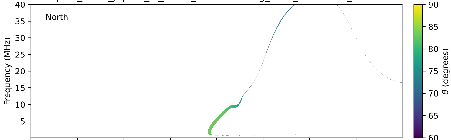
expres_earth_jupiter_io_jrm33_lossc-wid1deg_3kev_20251030_v11.cdf
