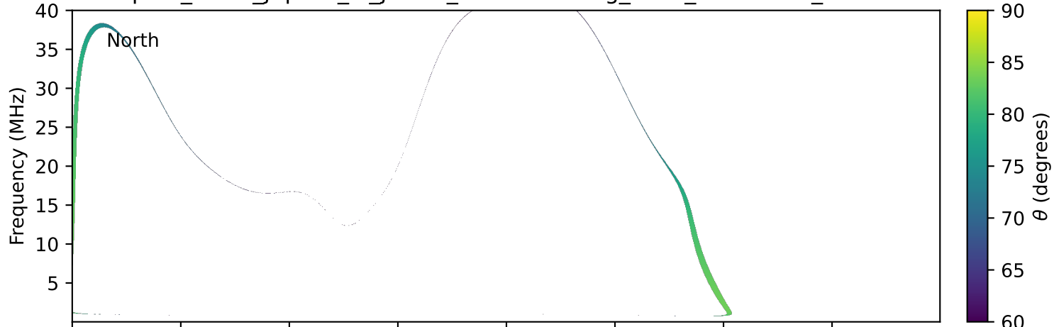
expres_earth_jupiter_io_jrm33_lossc-wid1deg_3kev_20251027_v11.cdf
