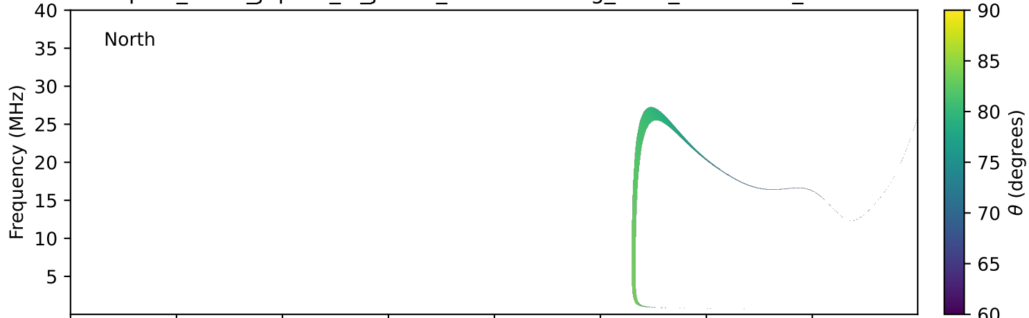
expres_earth_jupiter_io_jrm33_lossc-wid1deg_3kev_20251021_v11.cdf
