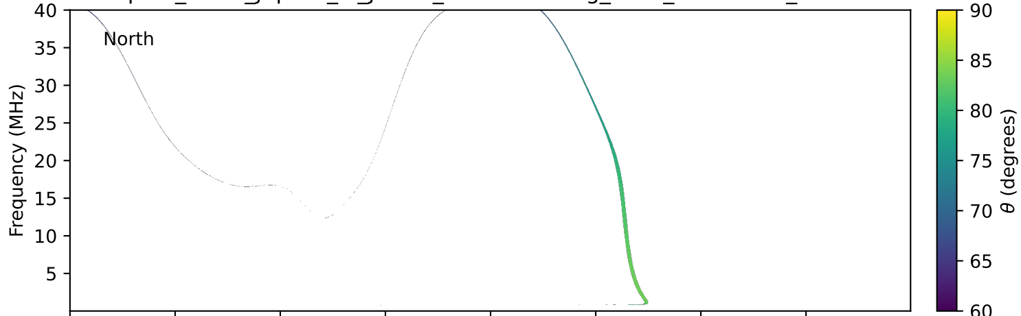
expres_earth_jupiter_io_jrm33_lossc-wid1deg_3kev_20251020_v11.cdf
