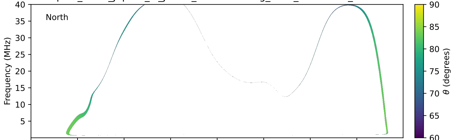
expres_earth_jupiter_io_jrm33_lossc-wid1deg_3kev_20251018_v11.cdf
