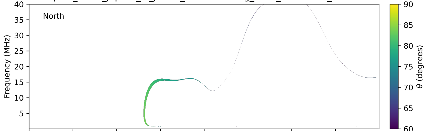
expres_earth_jupiter_io_jrm33_lossc-wid1deg_3kev_20251016_v11.cdf
