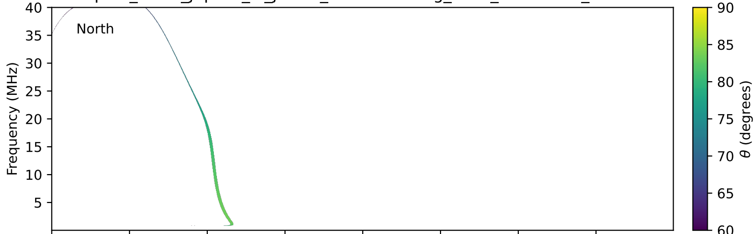
expres_earth_jupiter_io_jrm33_lossc-wid1deg_3kev_20251008_v11.cdf
