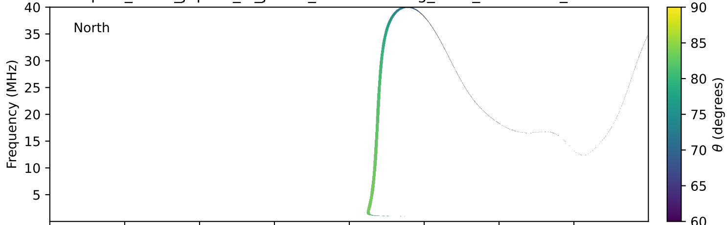
expres_earth_jupiter_io_jrm33_lossc-wid1deg_3kev_20251007_v11.cdf
