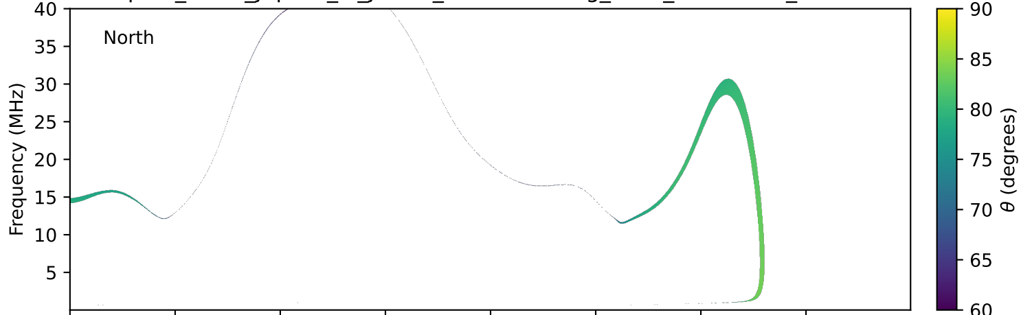
expres_earth_jupiter_io_jrm33_lossc-wid1deg_3kev_20251004_v11.cdf
