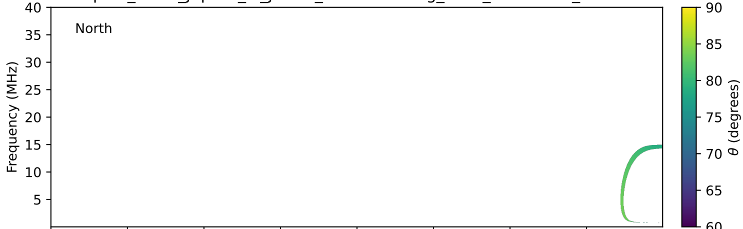
expres_earth_jupiter_io_jrm33_lossc-wid1deg_3kev_20251003_v11.cdf
