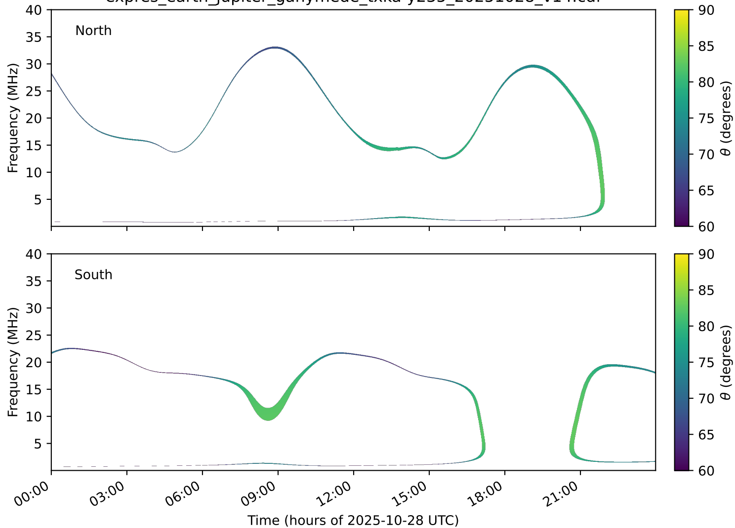
expres_earth_jupiter_ganymede_txka-y235_20251028_v14.cdf
