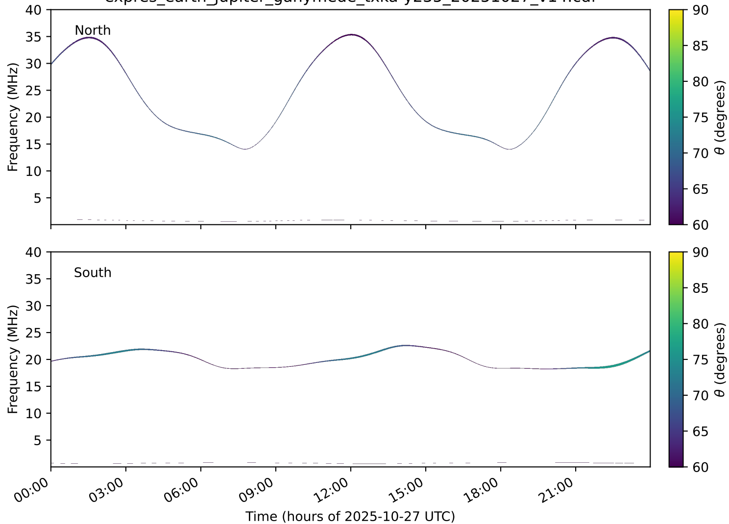
expres_earth_jupiter_ganymede_txka-y235_20251027_v14.cdf
