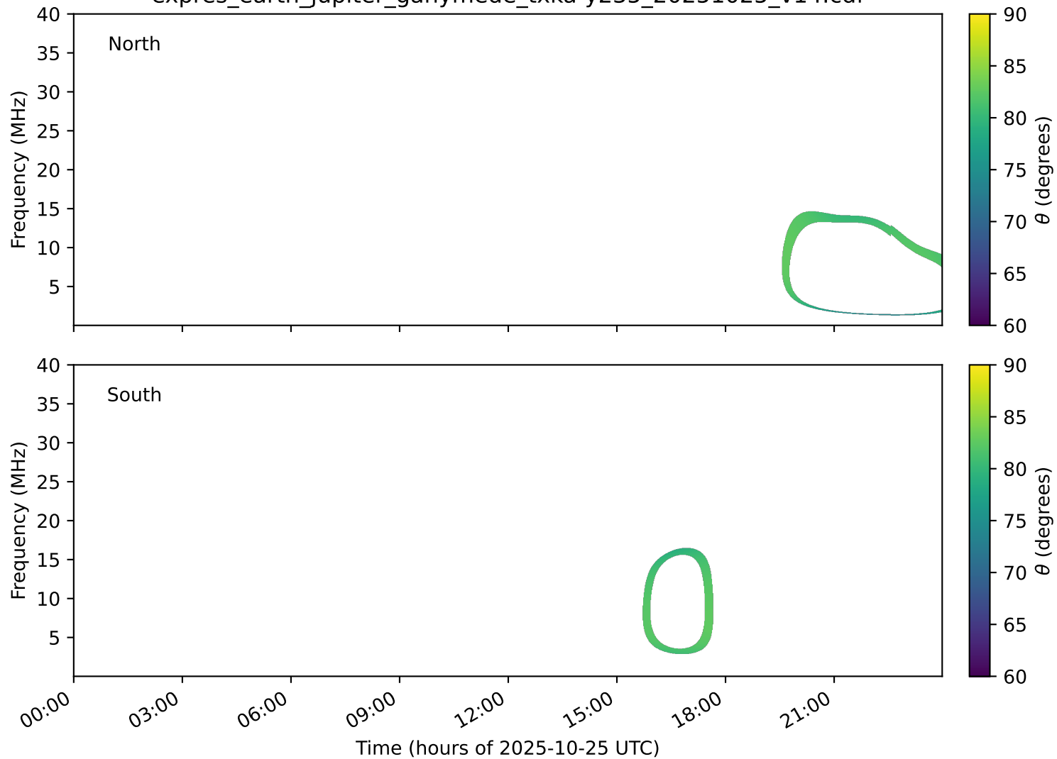
expres_earth_jupiter_ganymede_txka-y235_20251025_v14.cdf
