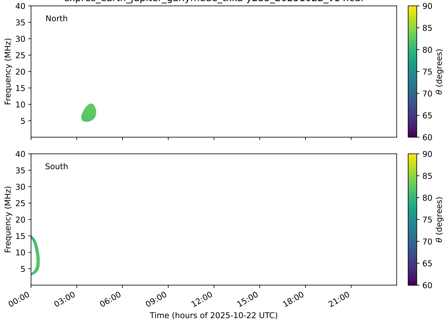
expres_earth_jupiter_ganymede_txka-y235_20251022_v14.cdf
