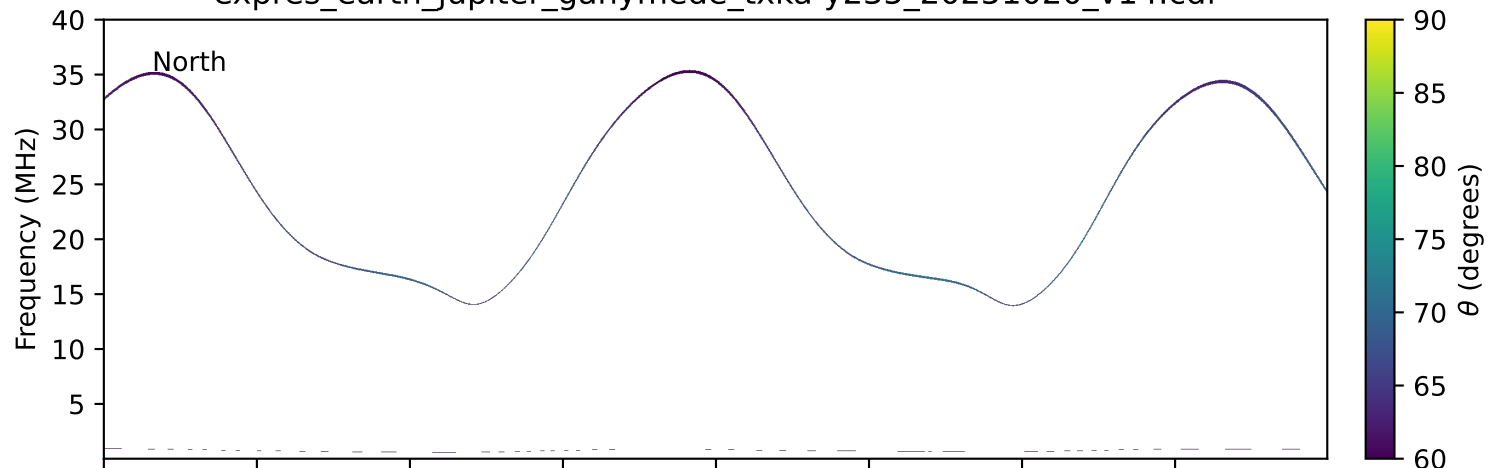
expres_earth_jupiter_ganymede_txka-y235_20251020_v14.cdf
