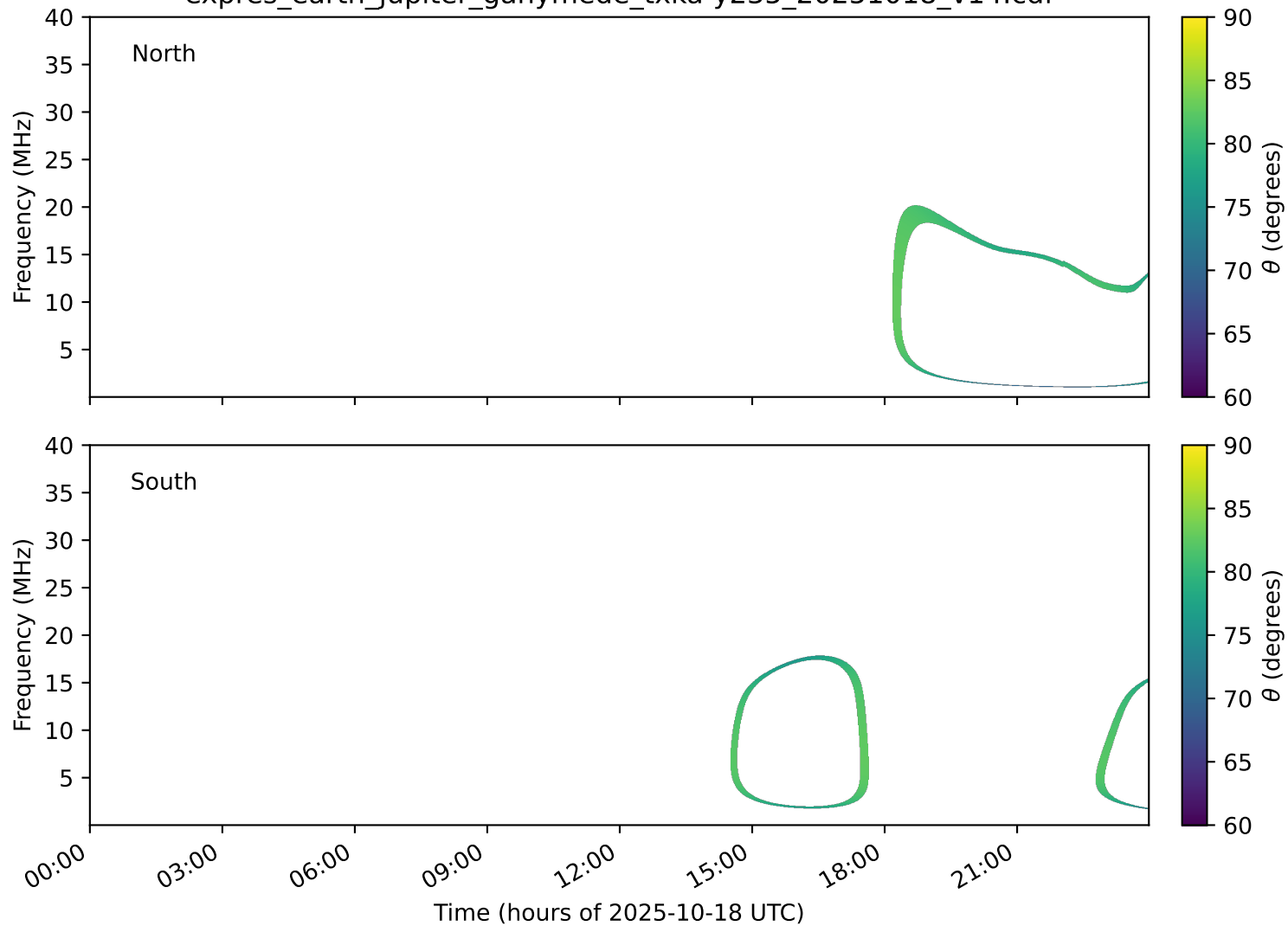
expres_earth_jupiter_ganymede_txka-y235_20251018_v14.cdf
