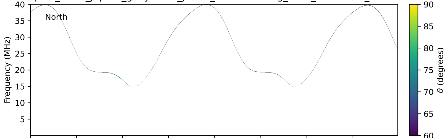
expres_earth_jupiter_ganymede_jrm33_lossc-wid1deg_3kev_20251020_v11.cdf
