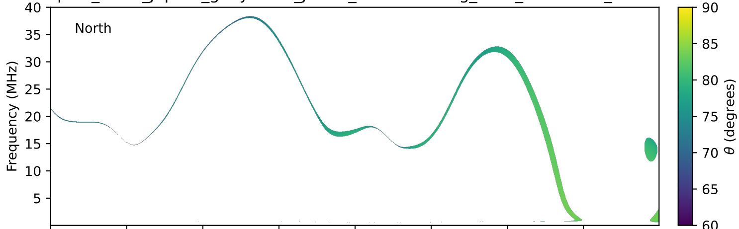
expres_earth_jupiter_ganymede_jrm33_lossc-wid1deg_3kev_20251014_v11.cdf
