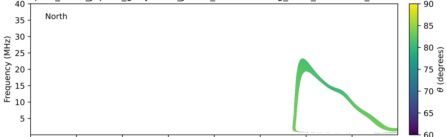
expres_earth_jupiter_ganymede_jrm33_lossc-wid1deg_3kev_20251011_v11.cdf
