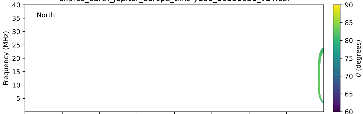
expres_earth_jupiter_europa_txka-y235_20251031_v14.cdf
