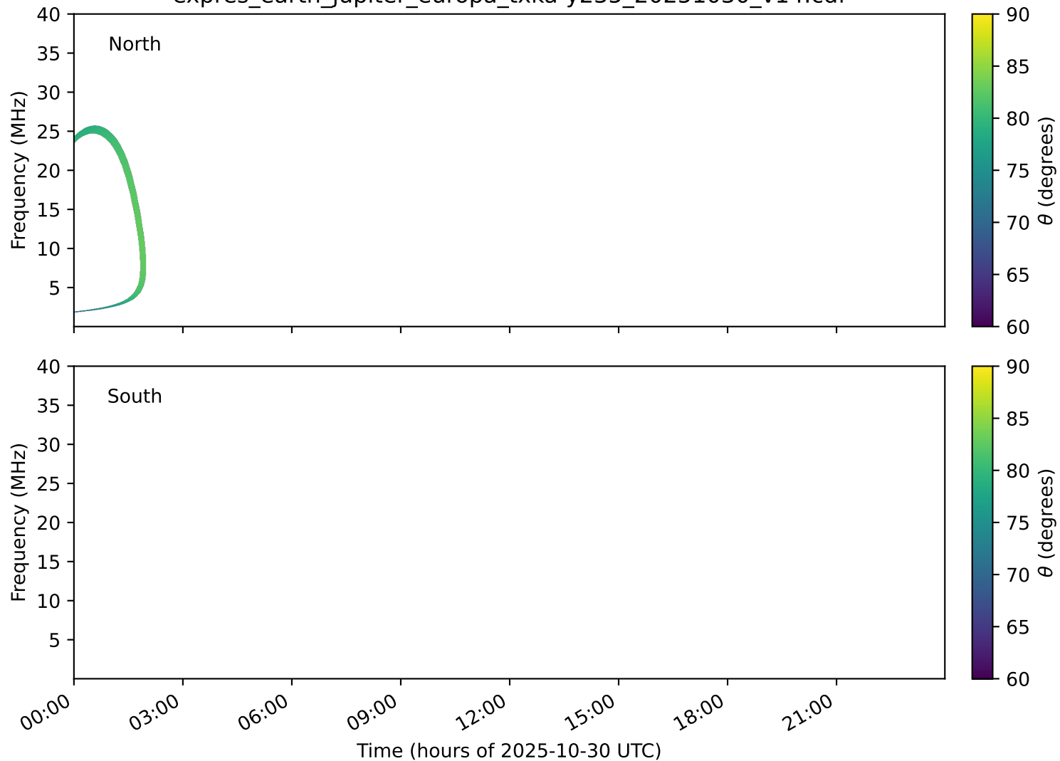
expres_earth_jupiter_europa_txka-y235_20251030_v14.cdf
