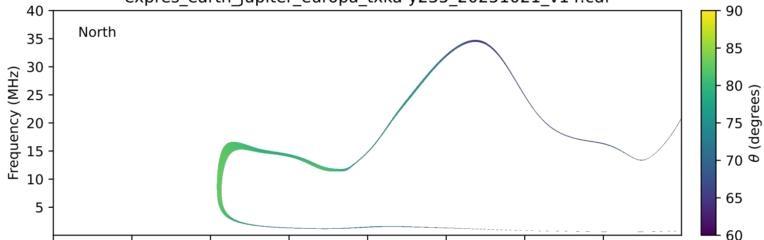
expres_earth_jupiter_europa_txka-y235_20251021_v14.cdf
