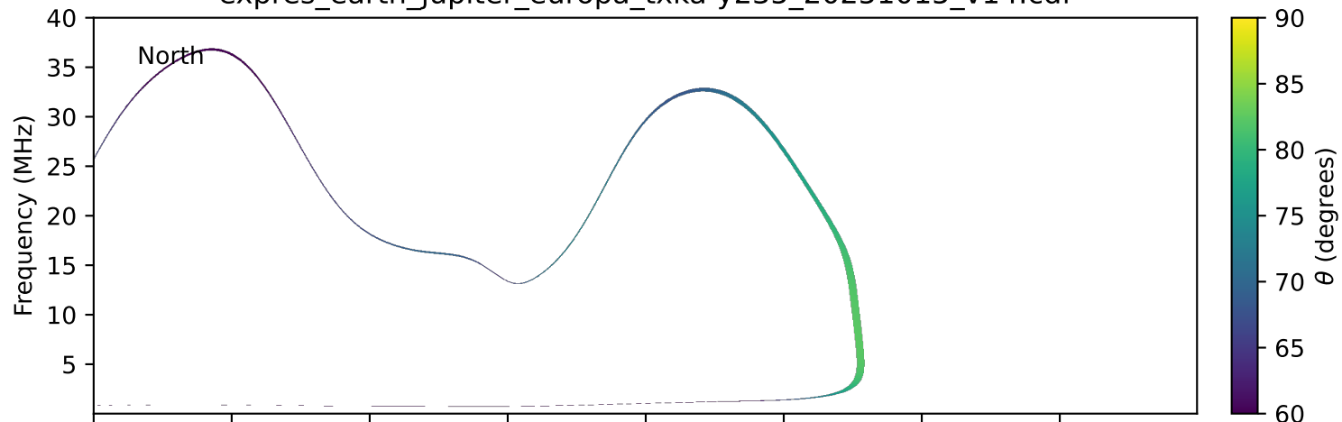
expres_earth_jupiter_europa_txka-y235_20251015_v14.cdf
