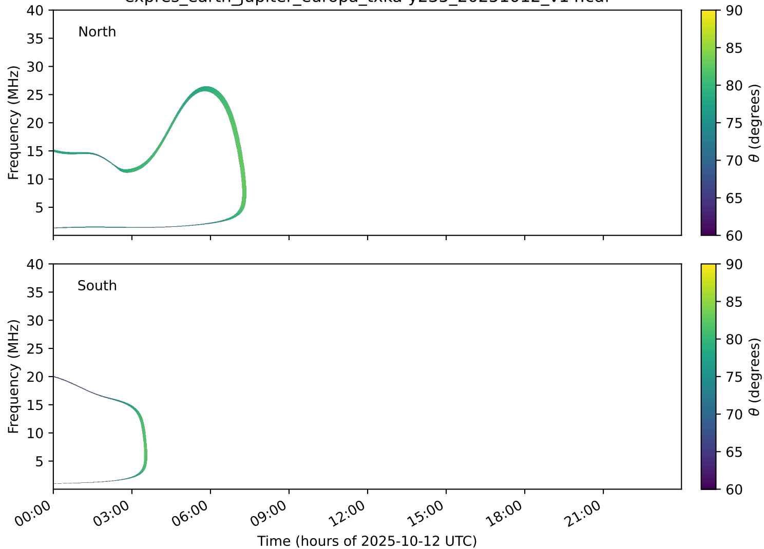
expres_earth_jupiter_europa_txka-y235_20251012_v14.cdf
