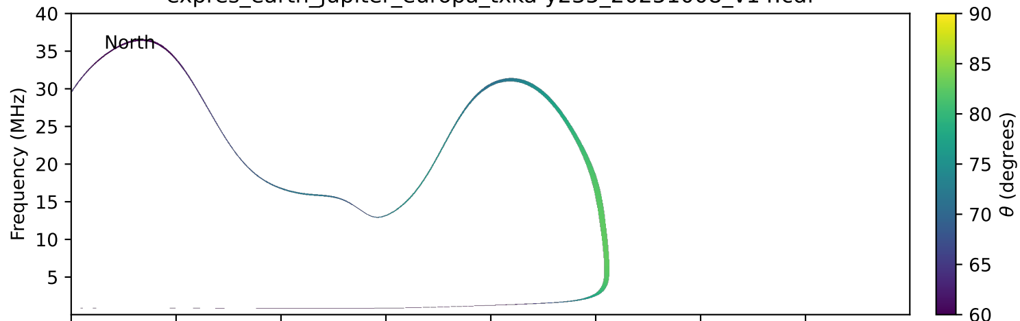
expres_earth_jupiter_europa_txka-y235_20251008_v14.cdf
