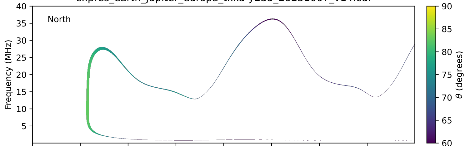
expres_earth_jupiter_europa_txka-y235_20251007_v14.cdf
