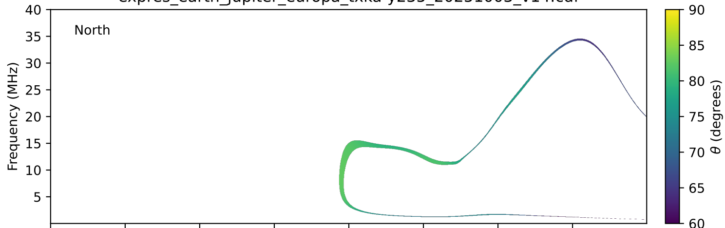
expres_earth_jupiter_europa_txka-y235_20251003_v14.cdf
